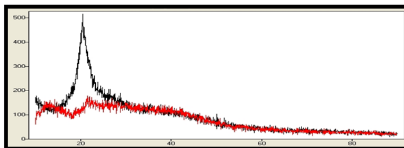
Fig 7. X-Ray Diffractogram of Alginate (red) and Chitosan (black) before the formation of nanoparticles
