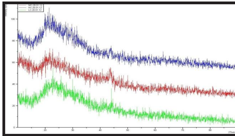
Figure 8 X-Ray Diffractograms of Nanoparticles with initial chitosan concentration of 0.05% (Green), 0.07% (Blue), and 0.09% (Red)
