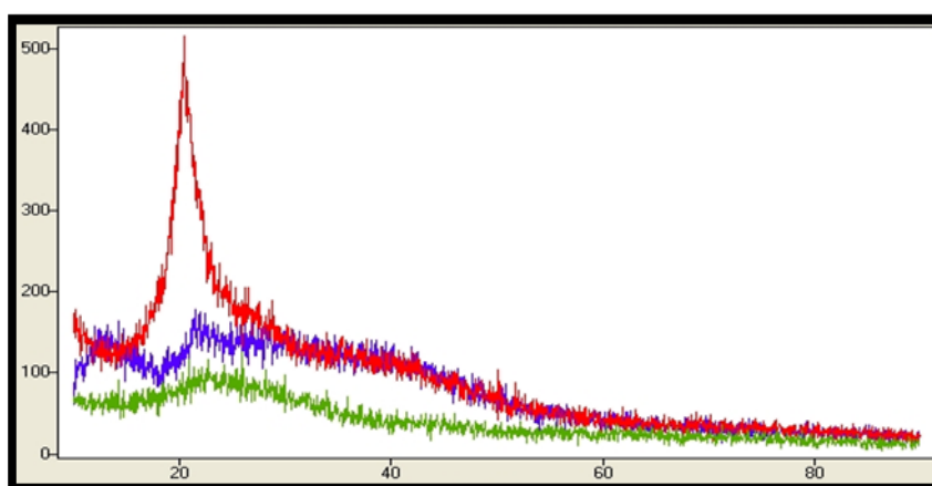
Fig 11. X-Ray Diffractogram of Chitosan (red) , alginate (blue)and Nanoparticles with Humulin N (green)
