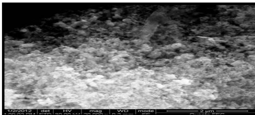
Fig 3. Scanning Electron Micrographs of Nanoparticles synthesized with initial chitosan concentration of 0.09%
