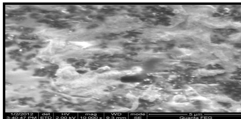
Fig 3. Scanning Electron Micrographs of Nanoparticles synthesized with initial chitosan concentration of 0.09%
