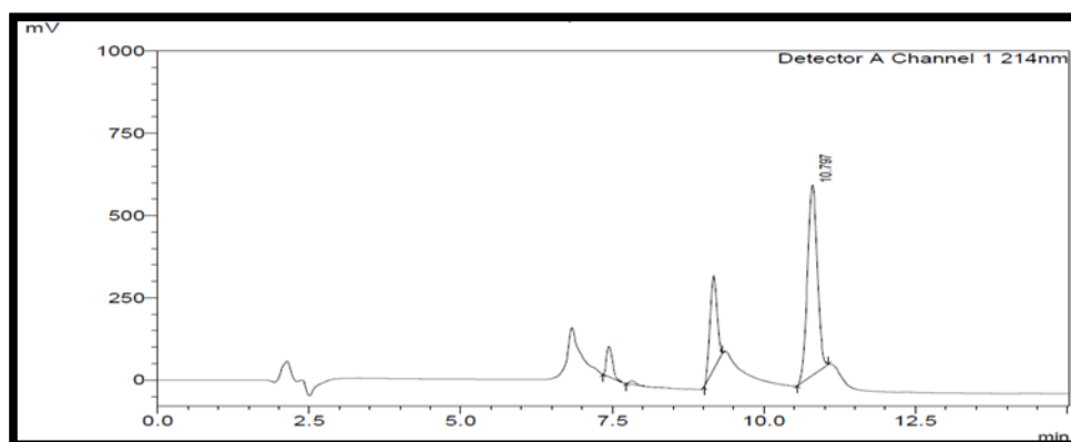
Figure 15 Chromatogram of Humulin N in simulated intestinal fluid
