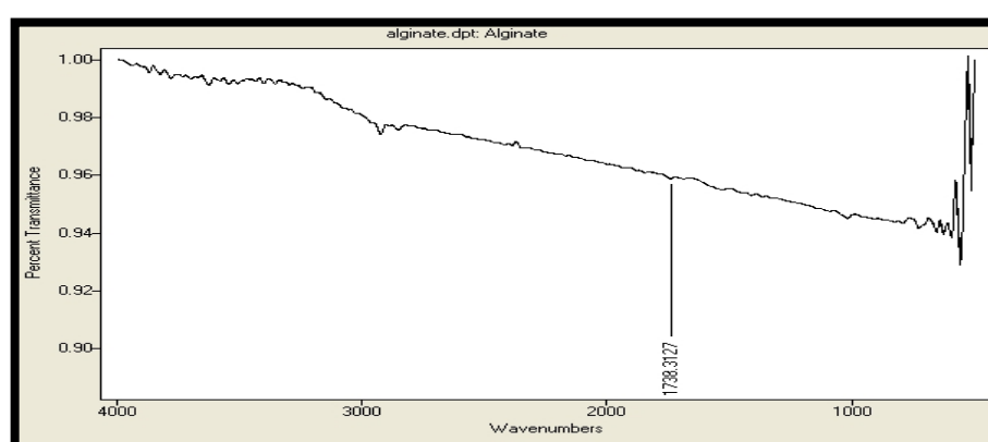
Fig. 5 FTIR spectrum of alginate
