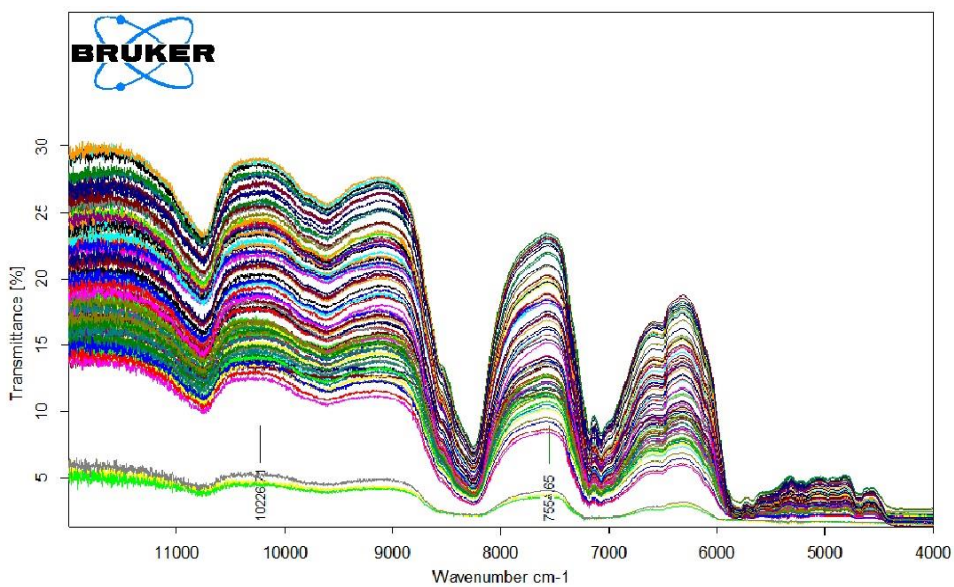
Fig.3 Spectrum of Ghee sample (Preprocessed)
