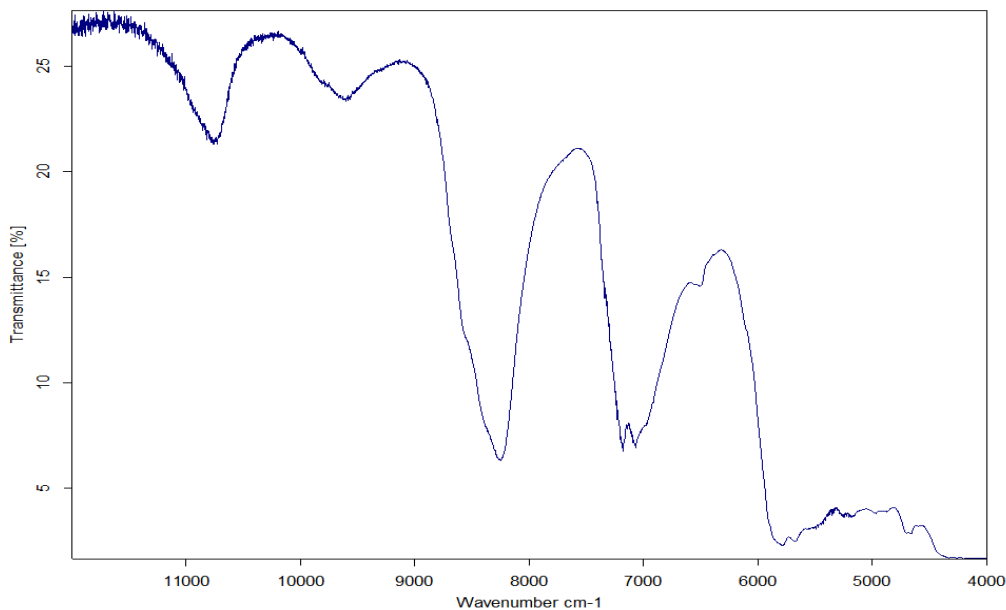
Fig.3 Spectrum of Ghee sample (Preprocessed)
