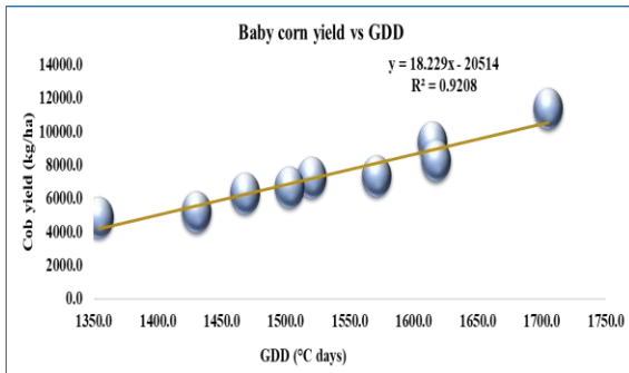
Fig 3c. Impact of GDD (°C days) on Baby corn yield
