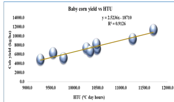
Fig 3d. Impact of HTU (°C day-hours) on Baby corn yield
