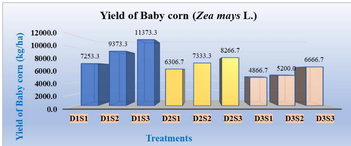
Fig 2. Yield of Baby corn ( Zea mays L.) during different sowing window
