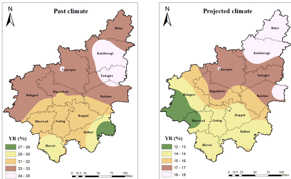
Fig 2. Spatial distribution of yield reduction (YR) in chickpea simulated in black clay soil under past (1991-2020) and projected (2021-2050) climate for all districts of NIK
