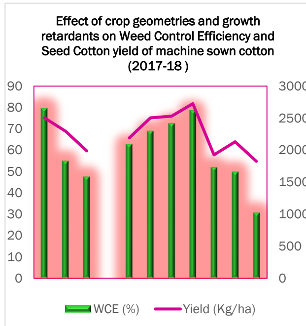
Fig . 1. Effect of crop geometries and growth retardants on Weed Control Efficiency and Seed Cotton yield of machine sown cotton (2017-18)
