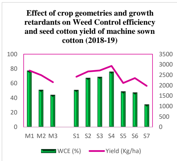
Fig. 2. Effect of crop geometries and growth retardants on Weed Control Efficiency and Seed Cotton yield of machine sown cotton (2018-19)
