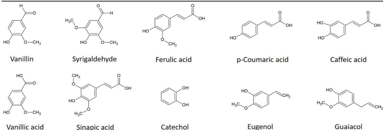
Fig 2. Structure of some commonly derived high commodity chemicals from lignin. (The structures are drawn using ACD ChemSketch software)
