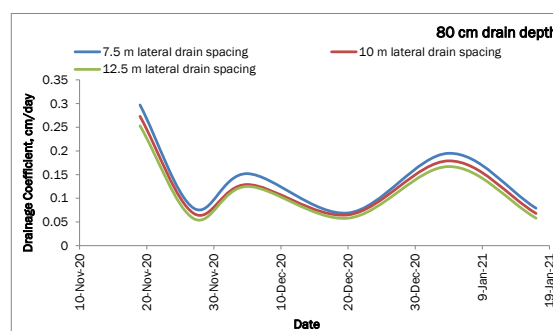
Fig.6 Drainage coefficient at 7.5, 10 and 12.5 m drain pipe spacing in 80 cm drain depth
